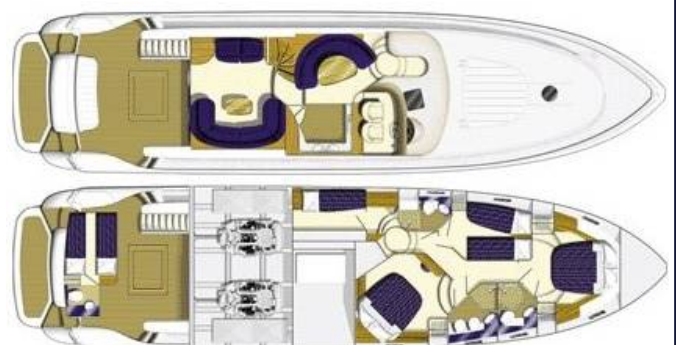
Lower deck with optional aft cabin
