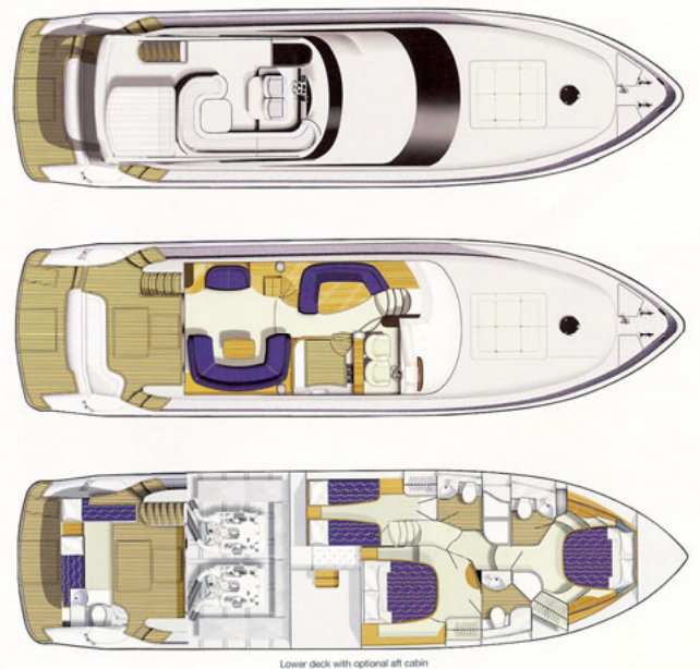
Lower deck with optional aft cabin
