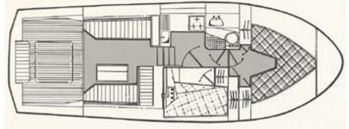
OPTIONAL STARBOARD CABIN ARRANGEMENT
