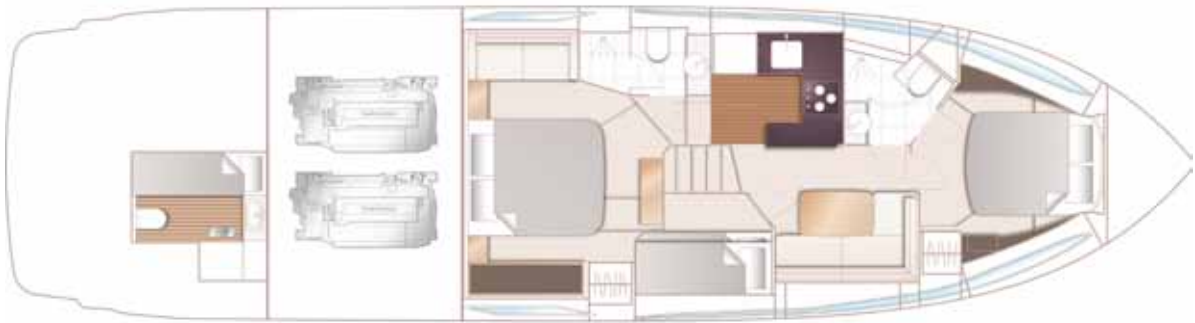
LOWER DECK
